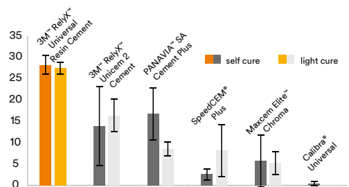
Shear bond strength (MPa) to dentin after artificial aging
